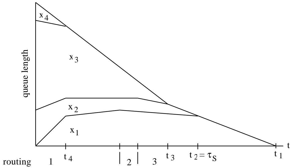
Fig. 3. A fluid trajectory for example 4. \lambda = 2 , \mu = (0.5, 0.5, 1.5, 1) , c = (1, 2, 4, 5) .
