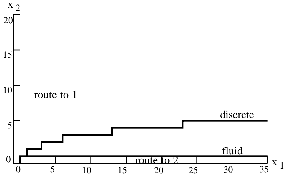
Fig. 1. Switching curves for example 1. \lambda = 1, \mu = (0.65, 0.65), c = (1, 2) .
