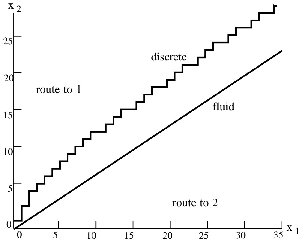
Fig. 1. Switching curves for example 1. \lambda = 1, \mu = (0.65, 0.65), c = (1, 2) .
