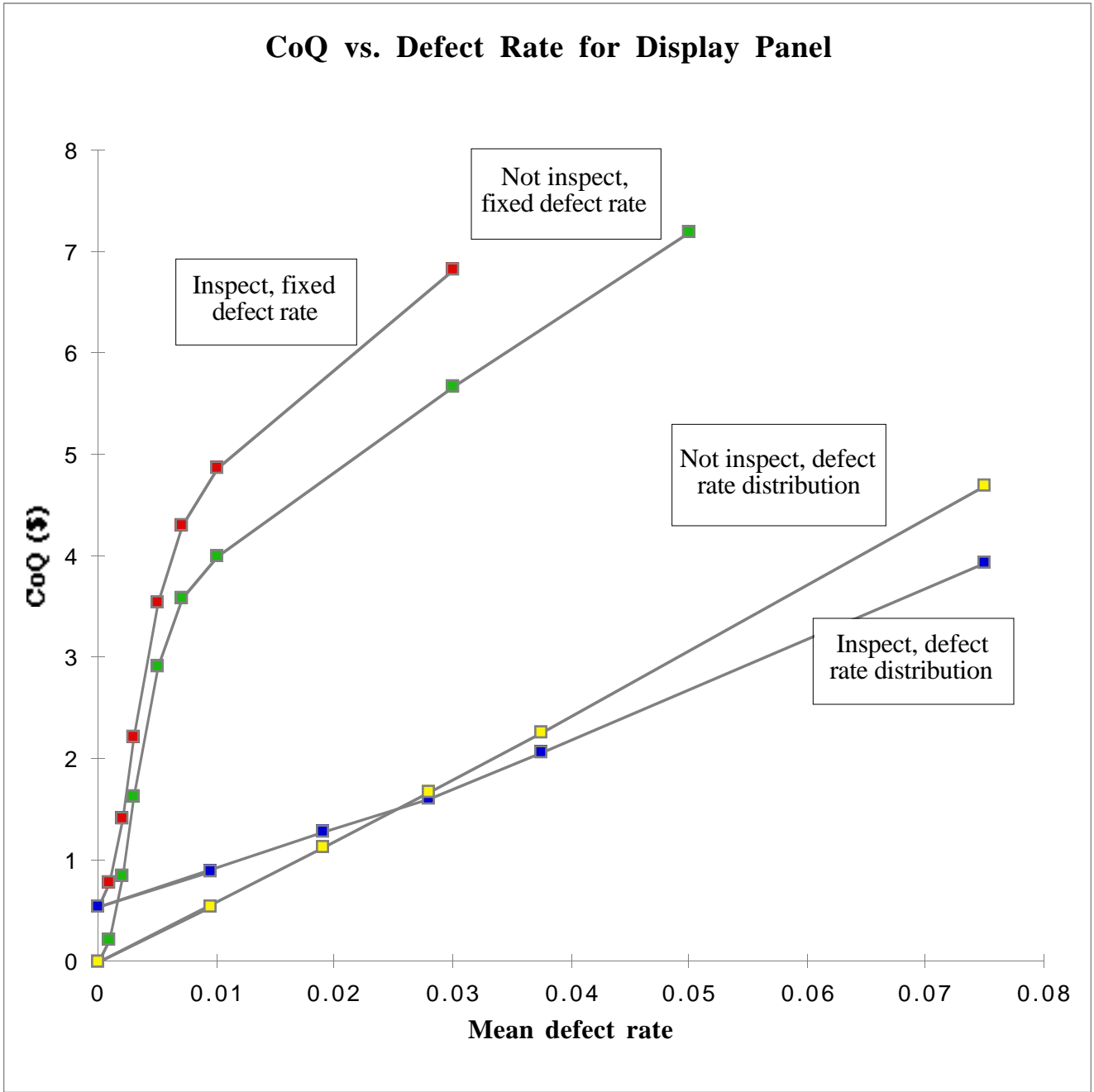
Figure 3. CoQ vs. Defect Rate for Display Panel
