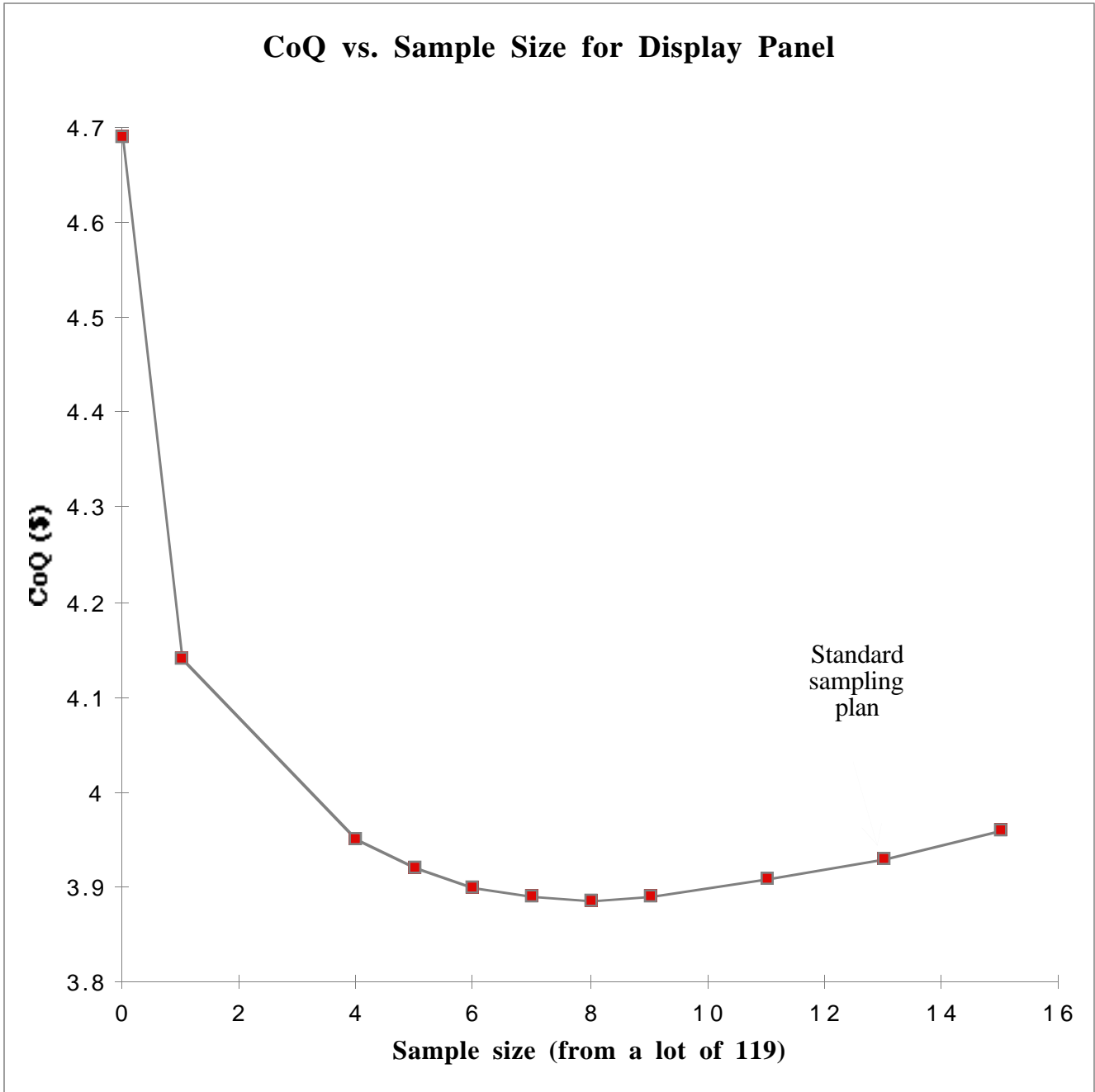
Figure 4. CoQ vs. Sample Size for Display Panel
